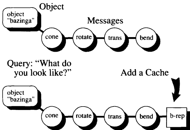
Figure 4: An inquiry adds a cache to the end of a list of messages. Here, the cache is of a boundary representation (b-rep) of the object.
